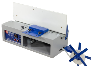
COLADEIRA HORIZONTAL 500
